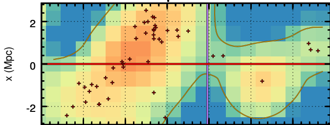
Sculptor Wall
